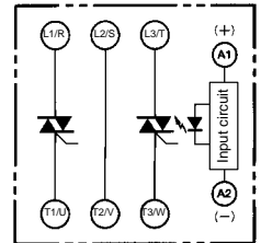
G3PB-□□□B-3-VD
