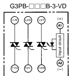
G3PB-□□□B-3-VD
