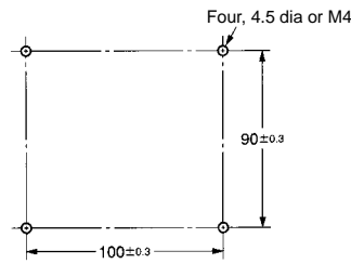
Mounting Holes
